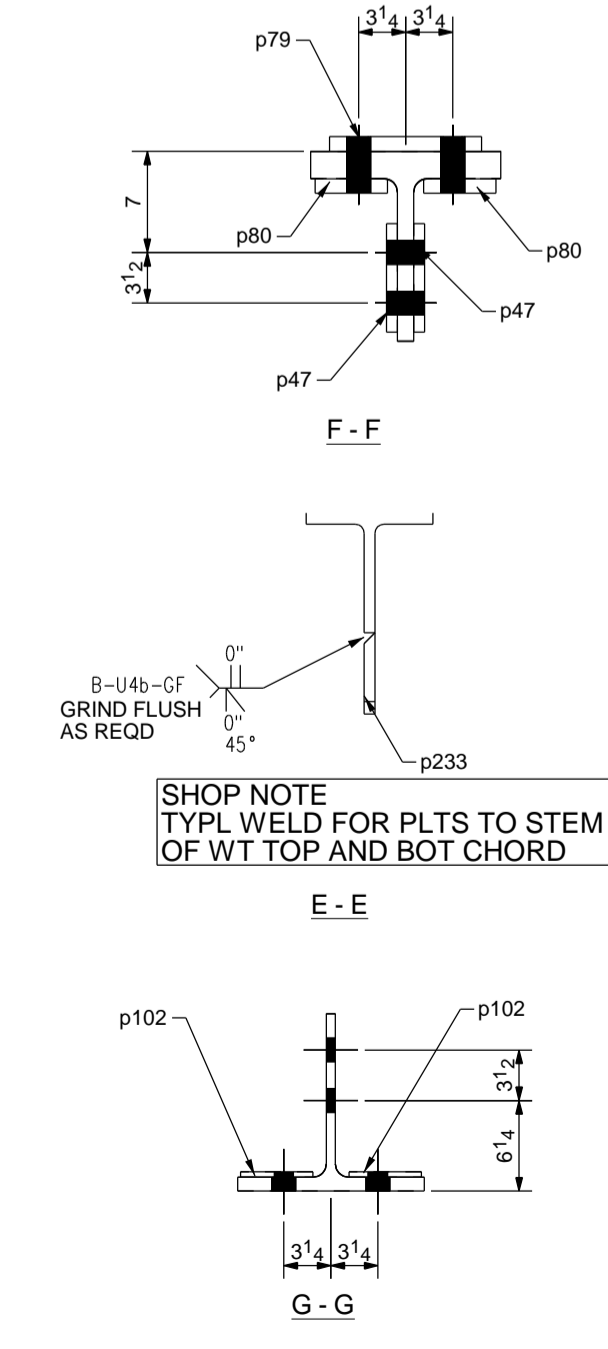
ONE - BEAM - 7T5 GRID LINE 8
